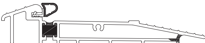
AM5 24mm Aluminium Threshold (for outward opening doors)
