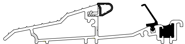
AM3 25mm Aluminium Threshold (for inward opening doors)
