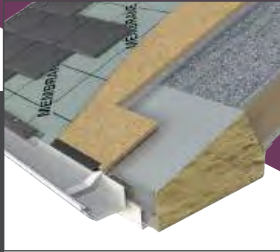
Fully insulated box beam eliminates the risk of condensation
