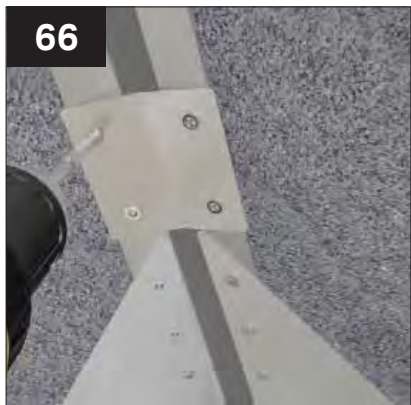
66 Fix the internal lower hip brace plate using 4 x CHAA 006 screws provided.
