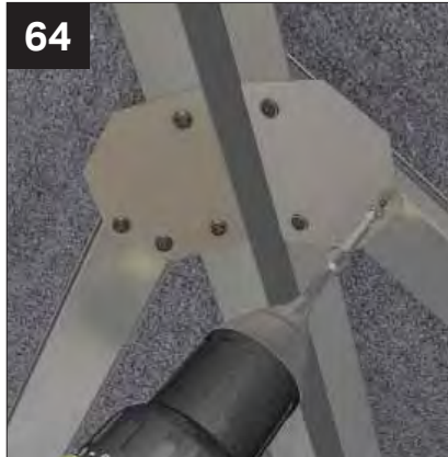
64 Where jack rafter abuts hip bar fix the jack rafter connection plates using 4 x CHAA 006 screws provided. NOTE: fit one screw through half clip that meets hip bar.
