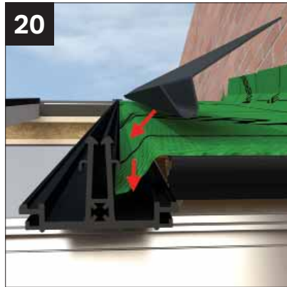
Where glazing is present, allow the membrane to overlap into the glazing bar as shown. The drainage channel can then be installed to clamp the membrane in place.
