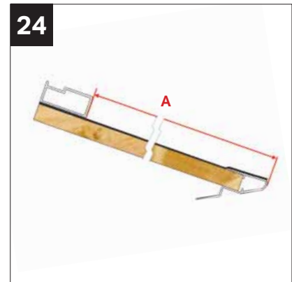
Dimension A given on critical dimension sheet. This gives distance from face of tile stop to outer edge of tile starter support.
