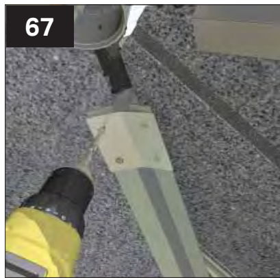
67 Fix the internal upper hip brace plate using 4 x CHAA 006 screws provided.
