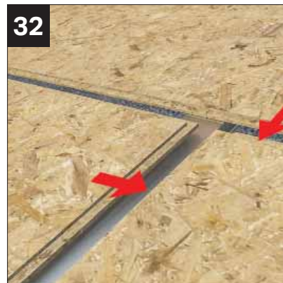
All OSB board edges are tongue and grooved to allow positive location. Continue to board from bottom to top (box beam to wall plate). NOTE: before fitting last row of OSB at the half ridge, ensure to fully insulate with supplied mineral wool between top of panels and host wall. See image (top right) page 11.
