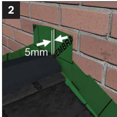
2 Centralise ridge to cap over apex. Position 5mm away from host wall. Foam fill void, prior to dress leading.
