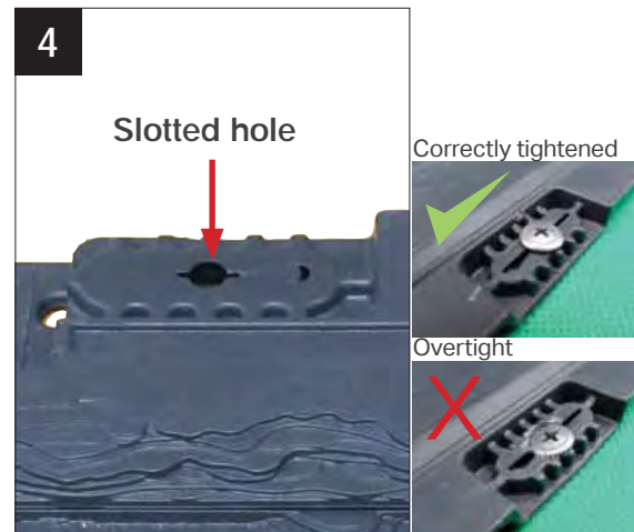
Repeat steps 3&4 following the fitting order guide until all starter strips are in place and are correctly fitted. Once correct, fully fix through slotted holes along the starter strips for permanent fix.
