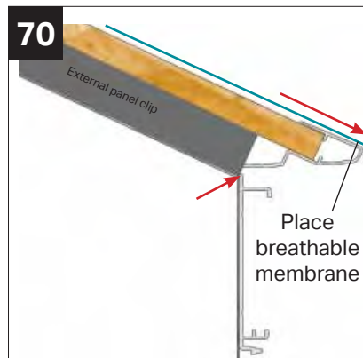
70 The breathable membrane is aligned to the front edge of the tile starter support.
