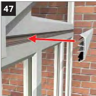
47 Fit internal and external gable stiffener claddings (if ordered)
