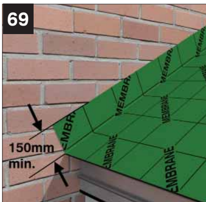
69 Start at eaves and position 150mm up the host wall. Place membrane (as step 70). Overlap each hip (as step 71).
