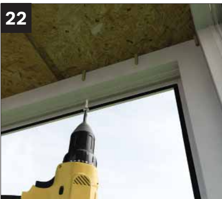
22 If packers used, recheck for being square, also check diagonals (corner to corner measurement). When these checks are complete finally secure by screwing up through head of frames into box beam. Fixings need to be within 200mm of each corner and at 450mm centres using, for example 4.8 x 80mm baypole screw NOT PROVIDED.
