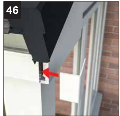
46 Fit 90° external corner cover trims
