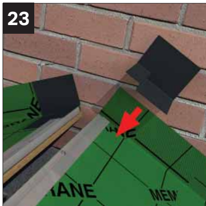
Fit the glazed ridge panel flashing trim to left and right side of ridge, (NRRI 011R right shown). These are bedded down using clear low modulus silicone.
