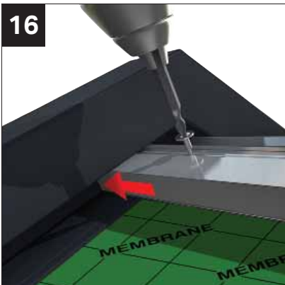
16 Slide tile stop under dry verge and fixed in place. See page 43 images 19 to 21 for details.
