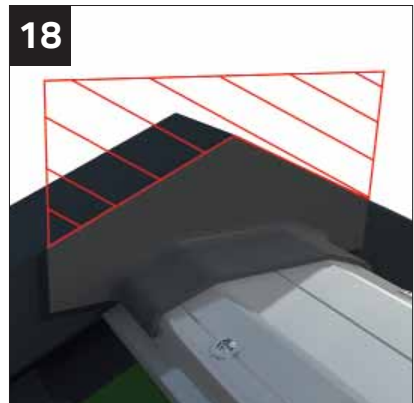
18 Fit the gable flashing. Mark and trim to fit the dry verge.
