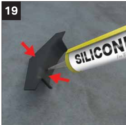
19 Apply clear low modulus silicone to the faces shown and refit.
