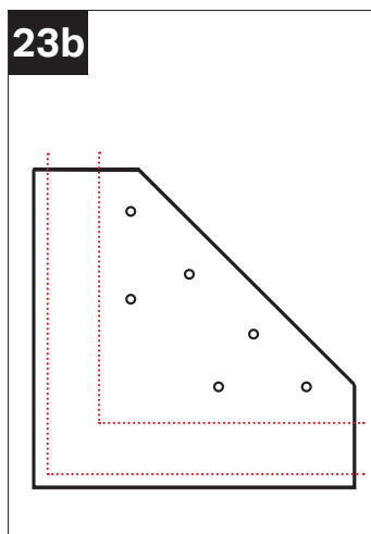
23b Fixing positions for standard soffit.
