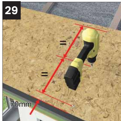
With OSB in position fix board 70mm up from tile starter support and 70mm down from upper edge followed by 1 x central fixing. NOTE: Fixing position at step 32.
