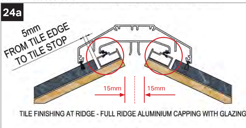
NOTE: CHECK FOR 30MM SPACE BETWEEN OSB BOARDS. THIS WILL ENSURE INNER TOP CAP SEALS ARE POSITIONED CORRECTLY ON THE TILES STOPS.
