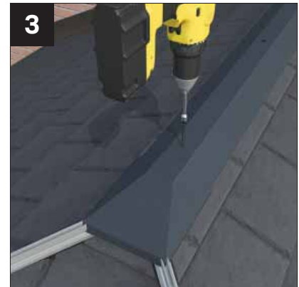
3 Fix ridge top capping using 5.5mm x 90mm (NRRSA 005BL) provided. Ensure hip spines are aligned with corners of ridge top capping.
