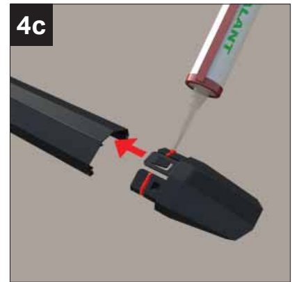
4c The hip bar top cappings at the radius end require (LMEC004) fitting, these require a bead of silicone applying prior to push fitting onto the end of each bar.
