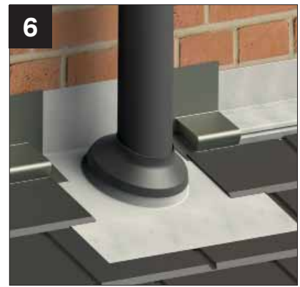
6 Cut the adjacent tile sheet allowing the pipe flashing apron to flow above the lower tiles as shown - this ensures the correct flow of any shedding water above the tiles.
