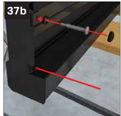
Fix the end cap in place using 2 x NRES 004 4.8 x 32 pan head screws with cover caps.
