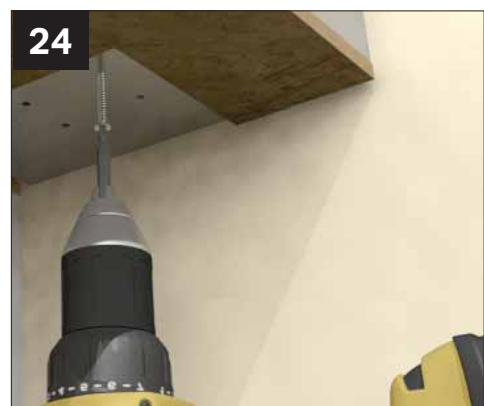
24 Fix up through the rear box beam wall brackets into the box beam using 6 x 50 x 50mm countersunk wood screws (RRX 025) provided. Finally ensure all box beam joints are fully sealed inside and out.
