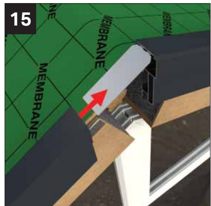
15 Fit opposite aluminium dry verge and point joints on upper and inner edges.
