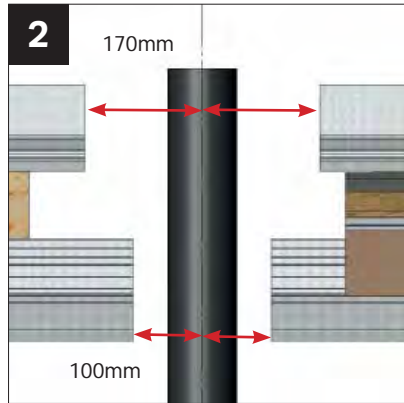
2 These should be installed in the usual manner paying attention to the setout dimensions as illustrated above
