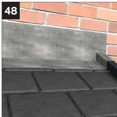
48 Lead flash to exiting host wall.
