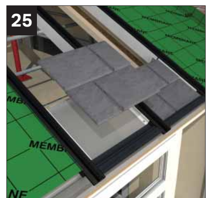
Position the box beam tile screens. Place in-line with adjacent tiling (not covering ventilation mesh) and secure with a single 4.2 x 25mm screw top centre (NRTS 050) provided.
