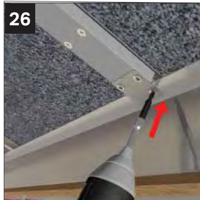
Finally secure to box beam support shelf the lower attachment plate using 4 x NRTS 050 fixings.
