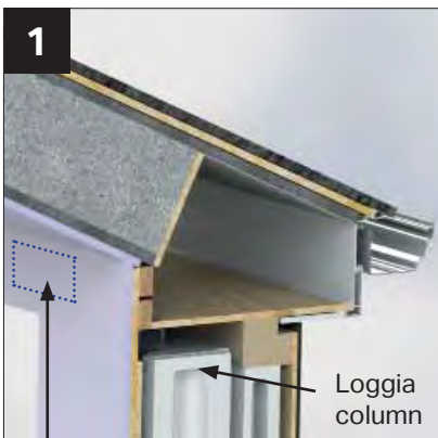
Double board adjacent to OSB cladding
