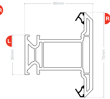
Midrail EWS 7056
