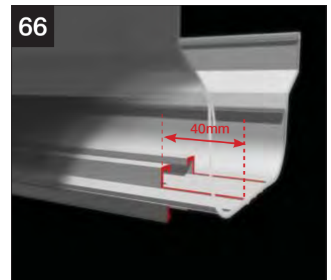
66 Now for the ridge top cap - Cut back the creasting channel on the top and the T bolt slot on the underside of the ridge top capping by 40mm.
