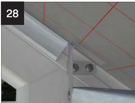
28 where panel adjacent to the gable is solid - the channel spans from insulated internal pelmet frame up to ridge detail and should be fitted directly below the 90mm insulation (insulated internal pelmet detail shown).
