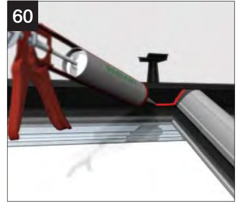
60 Seal around the top of each glazing bar top capping where it meets the rain baffle. Next, run a bead of sealant along the edge where the glazing meets the rain baffle.
