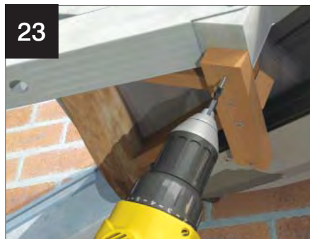
Fix into position using plasterboard screws. NOTE: when fitted, the battens should terminate at the centreline of the steel undercladding to allow for fitting of the adjacent panels
