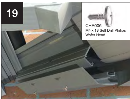
Fit valley plate at top of valley using fixings at max 250mm centres.
