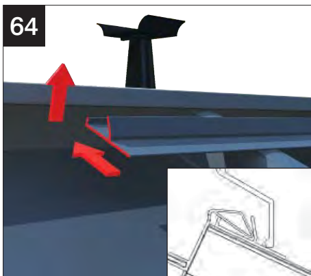
64 Then offer up the extrusion and attach to the rain baffle. Seal into soft touch moulded weathering shield and host wall.
