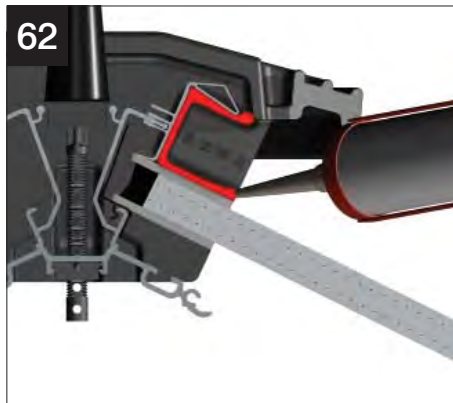
62 Run a bead of sealant in the position shown where the 'soft touch' moulded weathering tray meets the ridge body.
