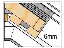
Slide remaining modesty panels into position, ensure that the batten on the screen is set 6mm back and screw fix to secure.
