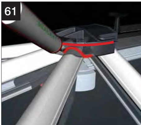
61 Seal around each glazing bar top capping where it meets the inner wall of the 'soft touch' moulded weathering shield. Also apply a bead of sealant to the top edge of the weathering shield so that the ridge capping will seal against it when fitted.
