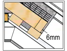
3 IMPORTANT: POSITION CLOAKING PANEL ASSEMBLY 6MM BACK FROM THE CROSS BATTEN (AS SHOWN) SCREW FIT INTO POSITION.
