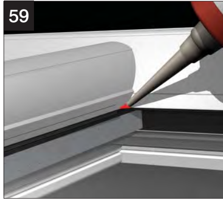
59 Carefully point the corners on each side of the capping where the gaskets abut each other.
