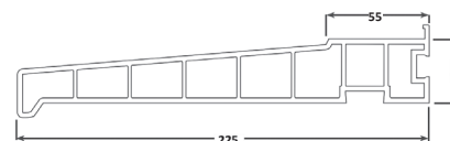
225mm cill
