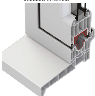
Standard threshold
