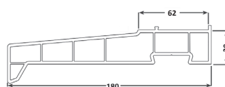
180mm cill
