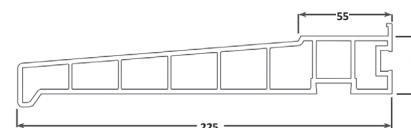
225mm cill
